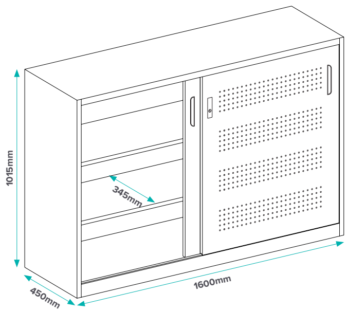
2 Shelves – 1600mm Wide
