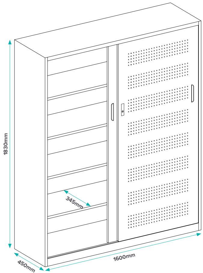
4 Shelves – 1600mm Wide
