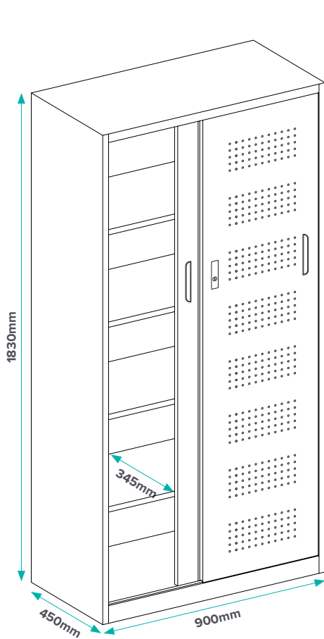
4 Shelves – 900mm Wide
