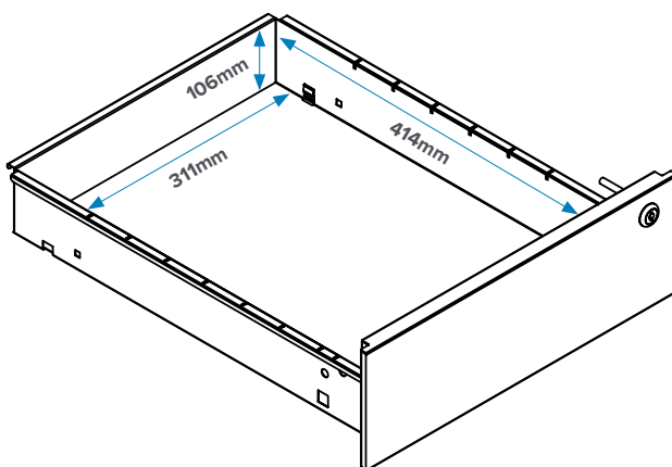
Box Drawer
