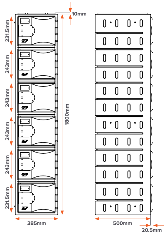
Full Height Six Tier
