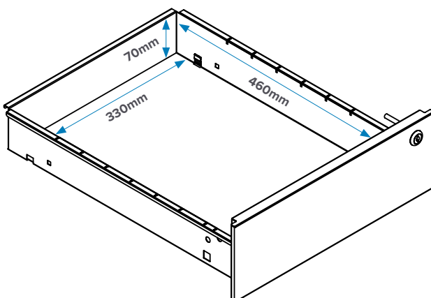
Box Drawer
